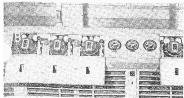
Figure 22. Water controls on front ledge of transmitter catwalk.
