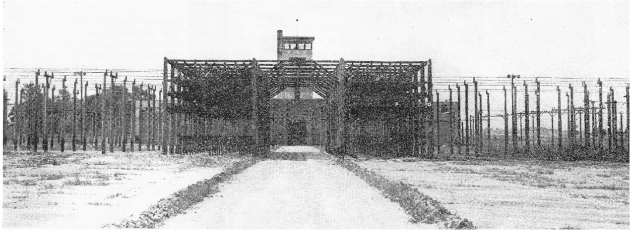
A view of the main antenna switching station with the transmission lines leading to the antennas.
