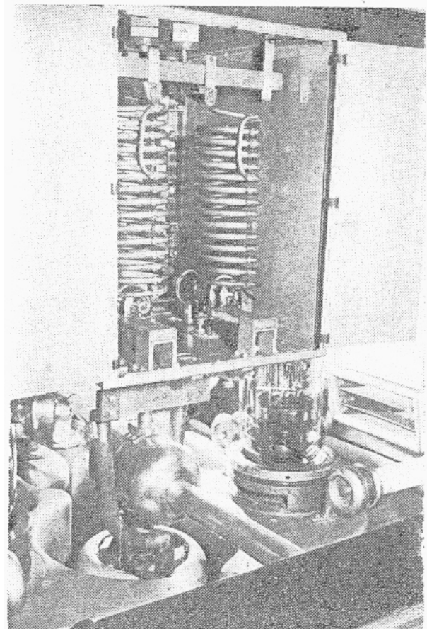
Figure 10. Interior of the power amplifier cabinet. Small cabinet between the two tubes provides shielding for grid circuits of amplifier.
