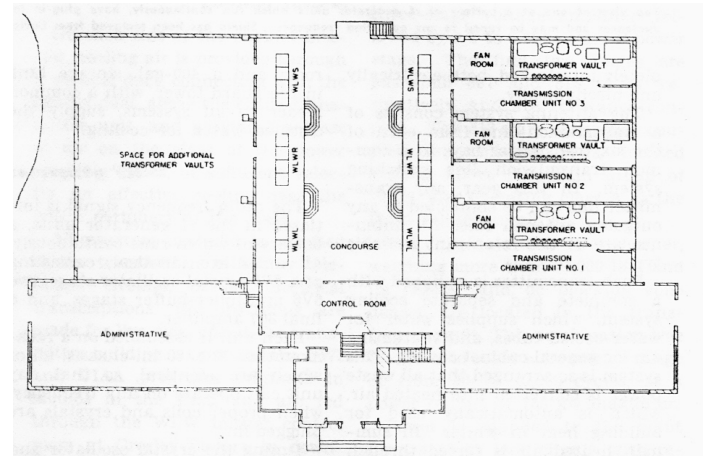
Figure 2. Floor plan of the transmitter building, showing the fireproof vaults where the high voltage transformers, filter reactors, filter condensers and high voltage control components are placed.
