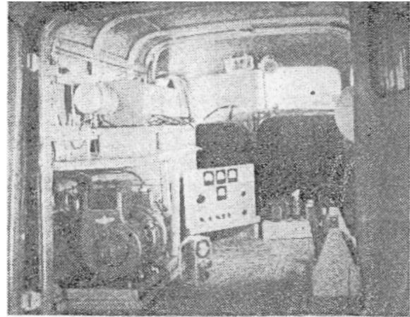
Figure 21. An interior view of the antenna service car. Equipment in this car includes two-way FM communications equipment, affording constant contact with the control room.
