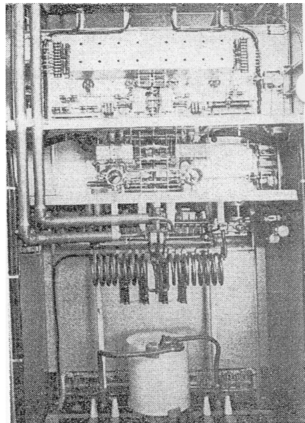
Figure 9. Output coupling adjustment, which is completed by swinging a small link coil into the field of the center of the driver plate inductance.
