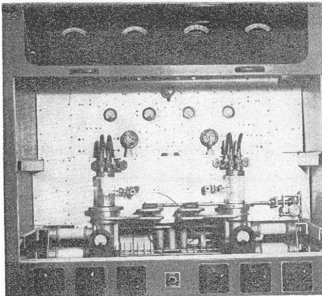
Figure 8. Front view of the RF driver which is composed of three stages. Each stage is separately tuned in both grid and plate circuits and is link coupled to the succeeding stages.
