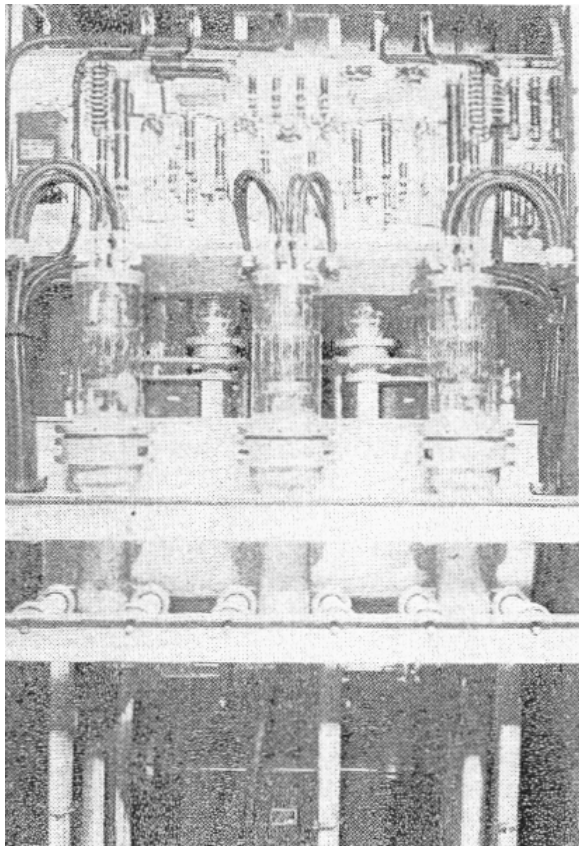
Figure 16. The 42 Ohm surge-limiting resistors which are in series with each modulator plate circuit, at bottom of unit in view below.
