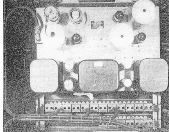
Figure 5. Rear view of one of the RF generators. Shield has been removed from second buffer stage coil to show construction.
