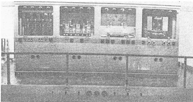
Figure 4. View of a section of the transmitter. Unit third from left is the RF driver which operates at carrier frequency throughout: range is 6-22 mc.
