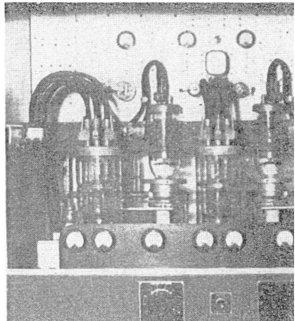
Figure 15. Modulator unit which consists of a three-stage voltage amplifier and a two to six-tube class B amplifier.
