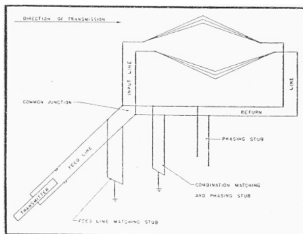
Figure 23. Rhombic antenna, showing reentrant feature and stub-tuning arrangement.
