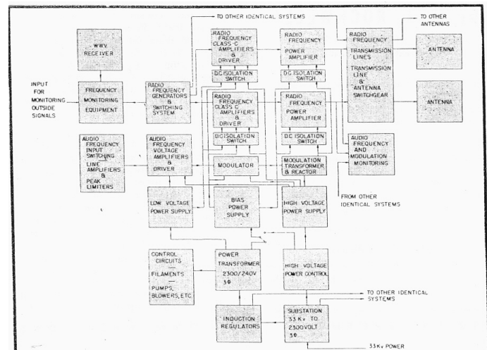
Figure 3. Block diagram of the complete transmission system.
