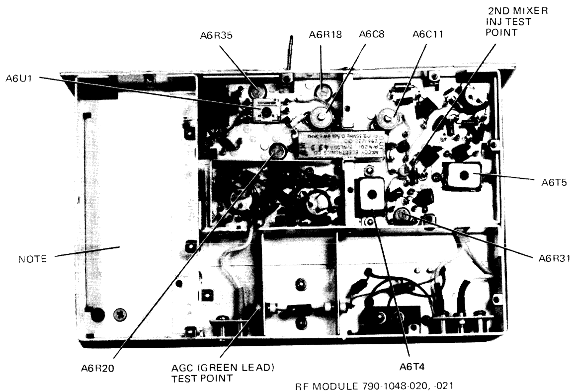
RF Module A6, Location of Test Points and Adjustments Figure 8
