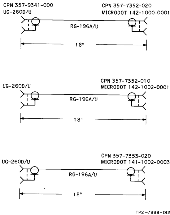
BNC to Subminiature Adapter Cables, Schematic Diagram Figure 1
